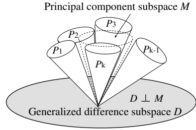
Fig. 2 Concept of generalized difference subspace
